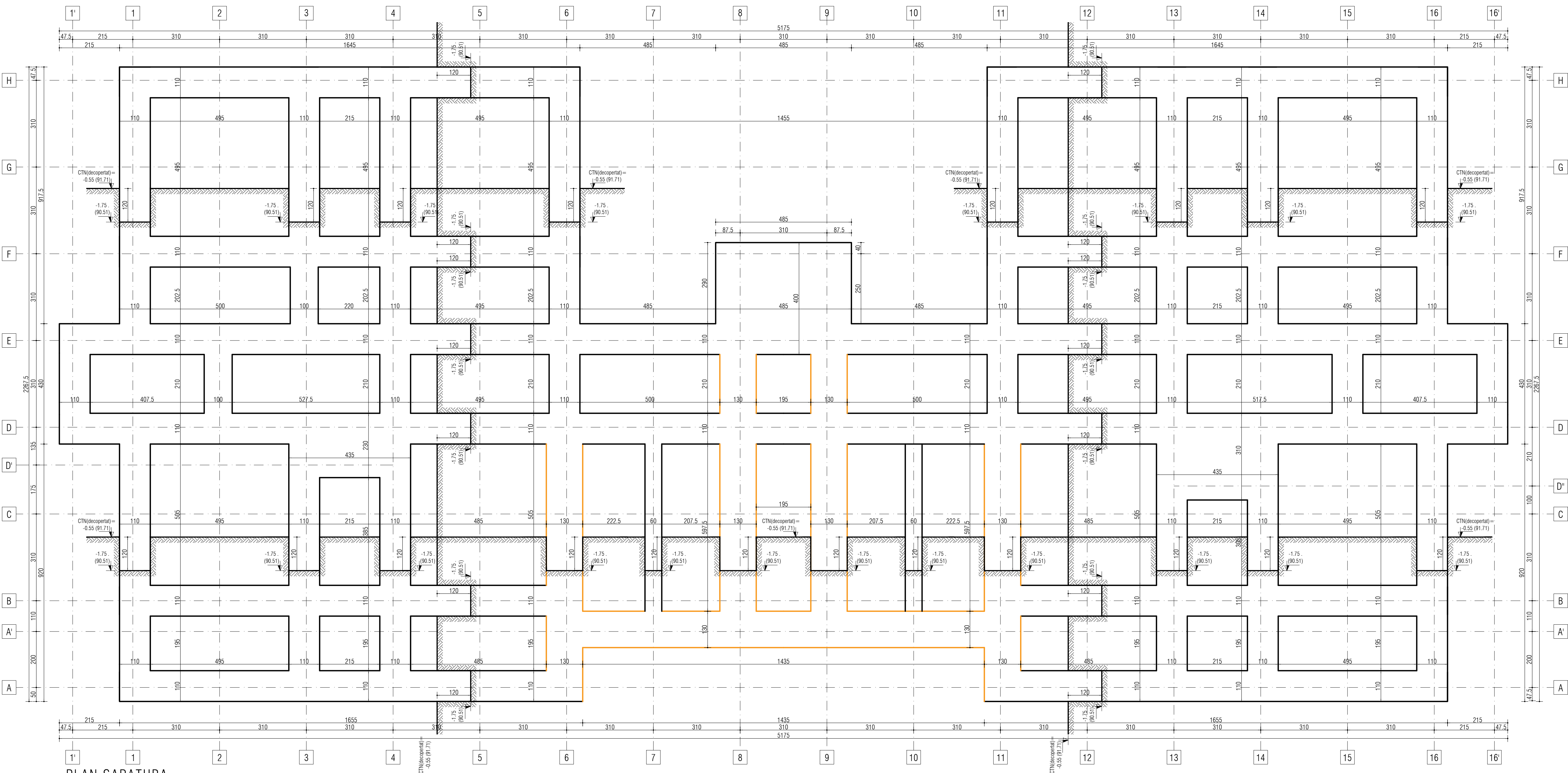
PLAN SAPATURA scara 1:75
