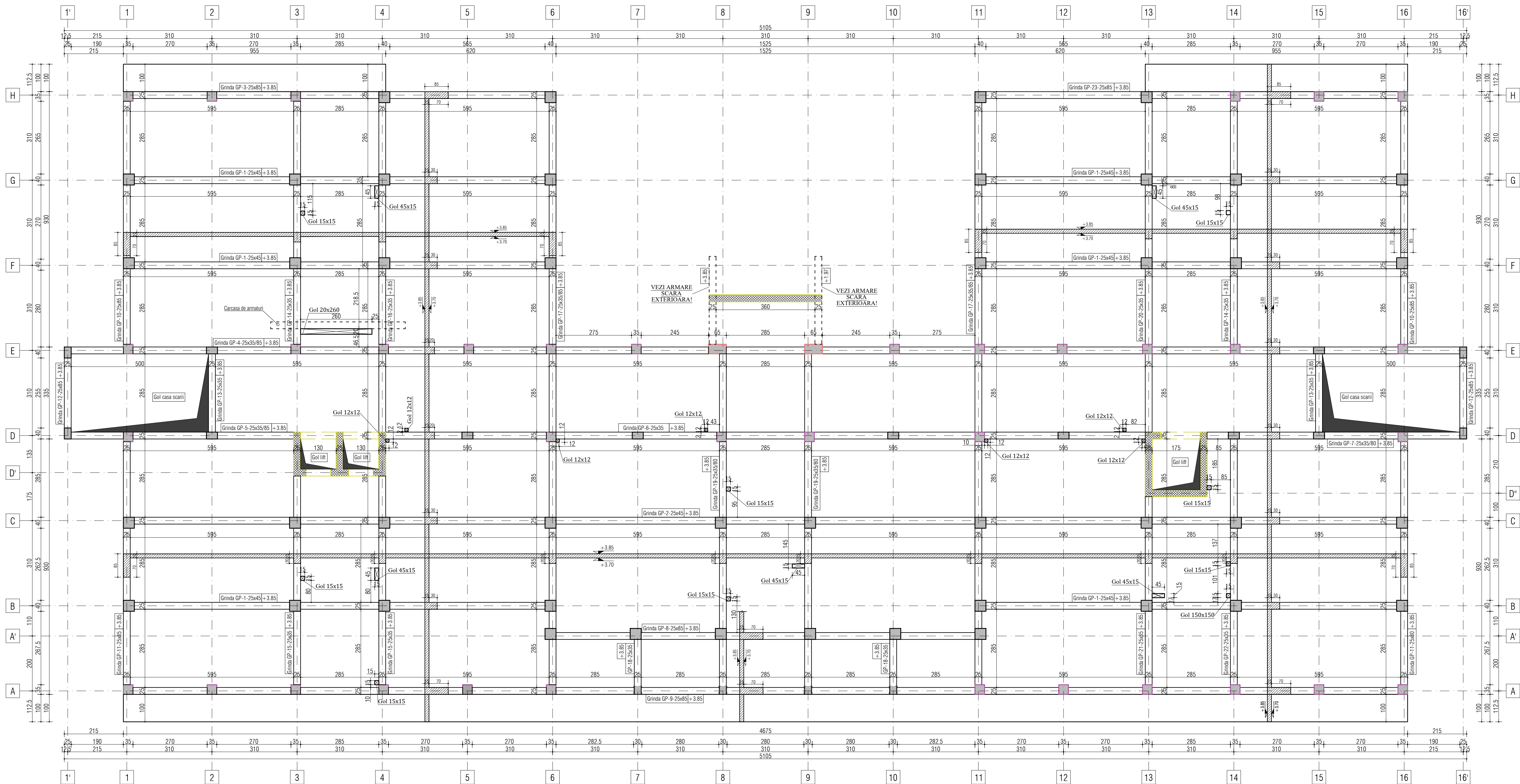
PLAN COFRAJ PLANSEU PARTER scara 1:75
