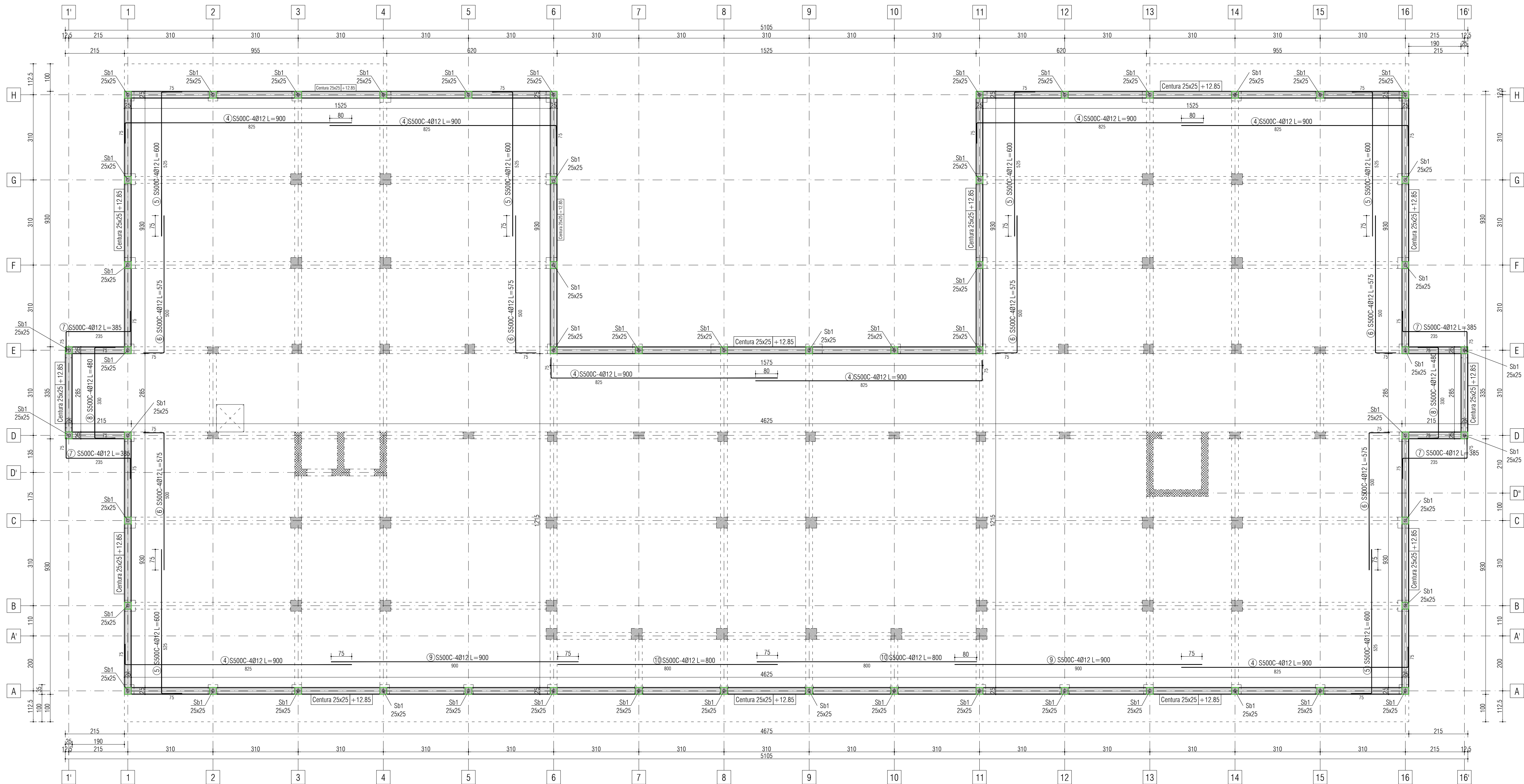
PLAN ARMARE ATIC cota +12.85 scara 1:75
